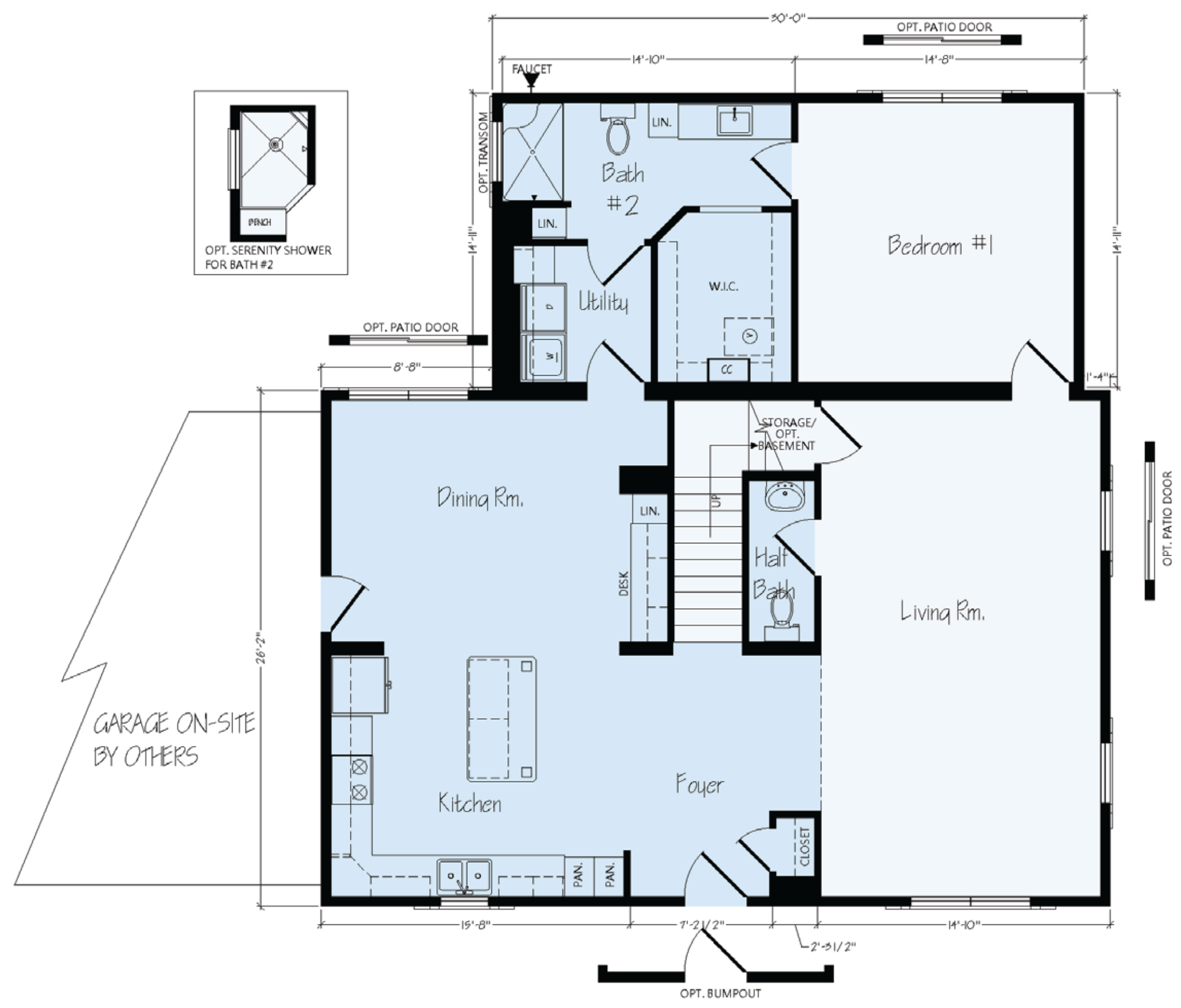
1ST FLOOR
